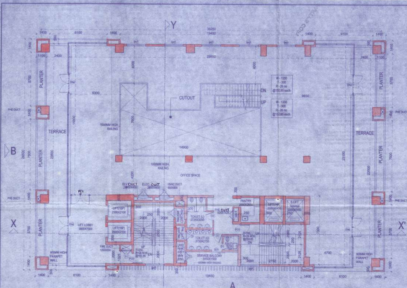
01 EIGHTH FLOOR PLAN (+42.85M LVL.) SCALE = 1:100
